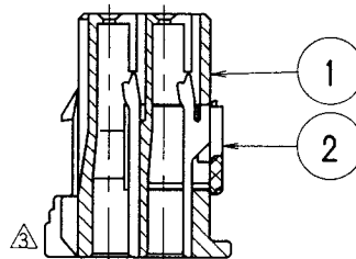
SEC. B-B
