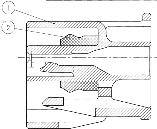
SEC. B-B
