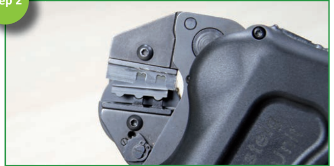
Select cable size as shown on top of crimp plate.
